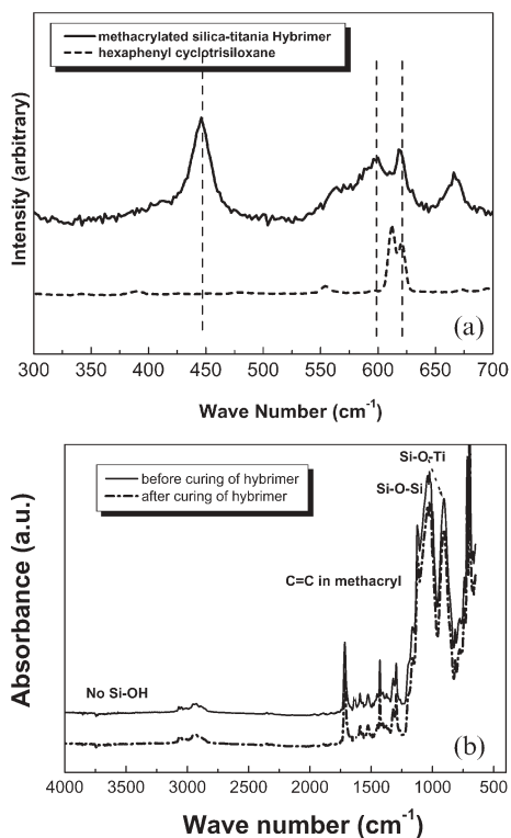
Fig. 2 FT-Raman spectra (a) and FT-IR spectra (b) of methacryl silica–titania hybridizer.
