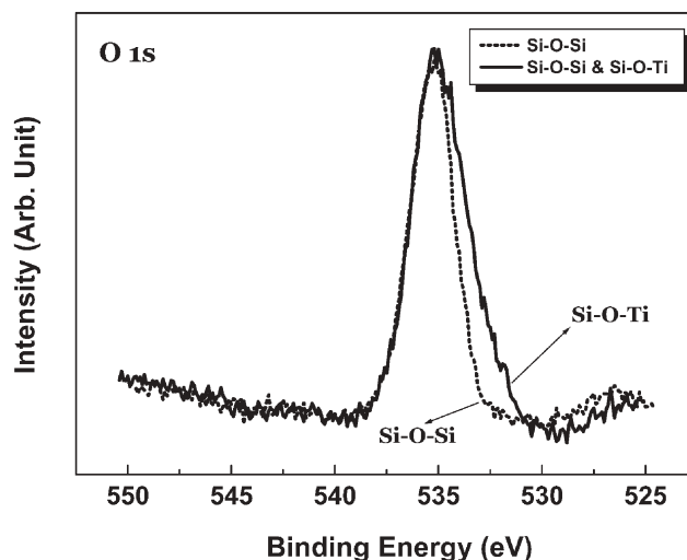
Fig. 3 Oxygen 1s XPS spectra of the methacryl silica–titania hybridizer, showing Si–O–Ti heterogeneous condensation.
