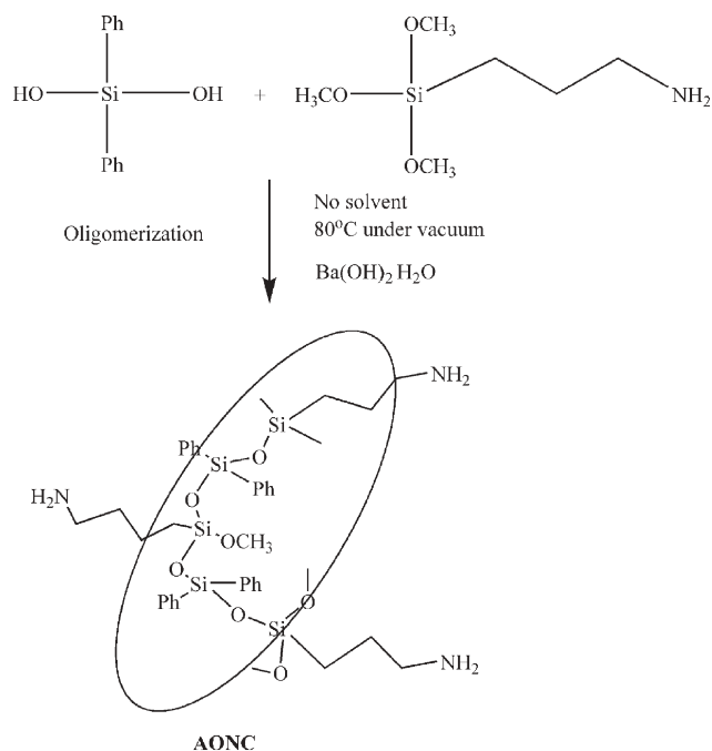
Scheme 1 The synthetic route and reaction scheme of AONC.
