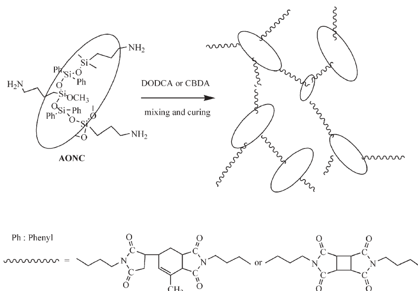
Scheme 2 The imide nanocomposite prepared from AONC and alicyclic dianhydrides as cross-linkers. The three-dimensional network structure in which each AONC is cross-linked by short diimide chains is shown.
